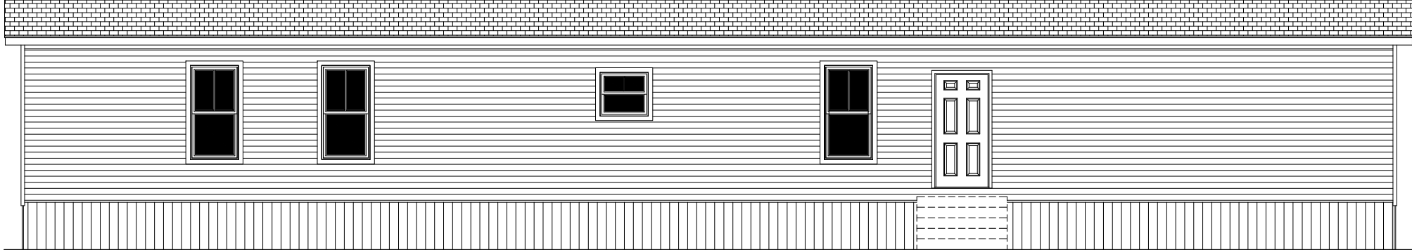
FRONT ELEVATION
