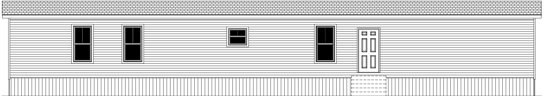
FRONT ELEVATION
